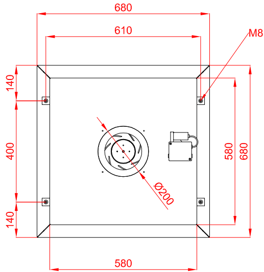
DIFVENT 6/6
